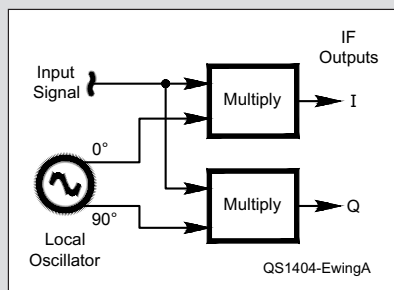
Figure A — In-phase and quadrature IFs.
