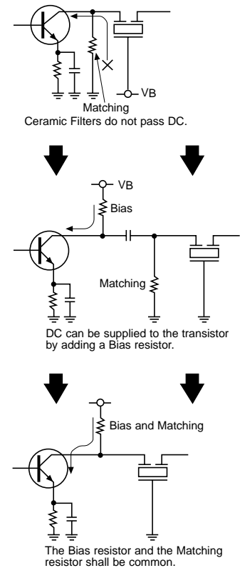
Fig. 433-13 Coupling With A Transistor
