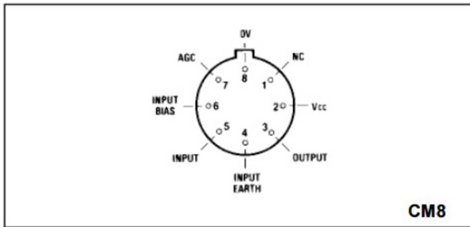
Fig.1 Pin connections (top view)
